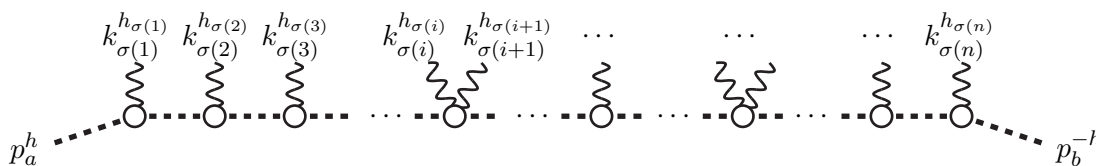
Figure 3: Tree-level scalar Feynman diagram.
