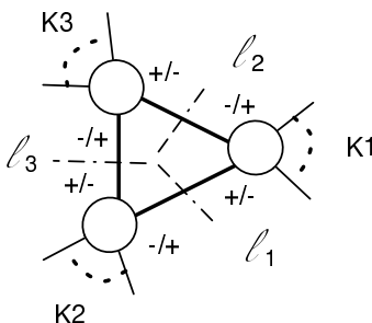
Figure 6: The triple-cut contribution the amplitude.
